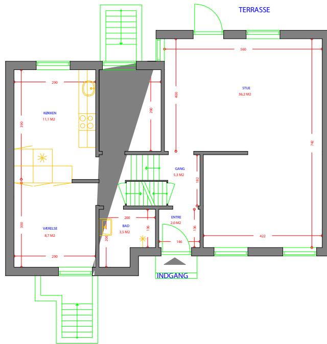
AFDELING 10 TYPE 46 4 RUMS 110 M2 STUEPLAN
