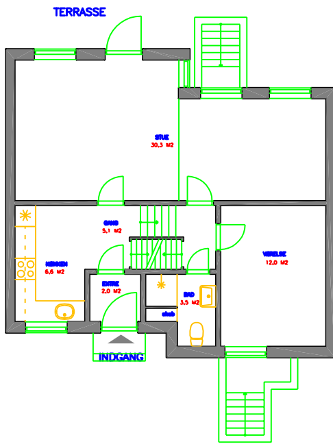
AFDELING 10 TYPE 34 3 RUMS 98 M2 STUEPLAN
