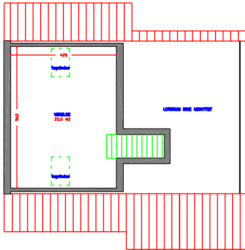
AFDELING 10 TYPE 34 3 RUMS 98 M2 TAGPLAN
