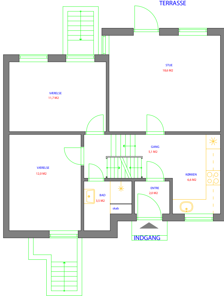
AFDELING 10 TYPE 33 3 RUMS 73 M2 STUEPLAN
