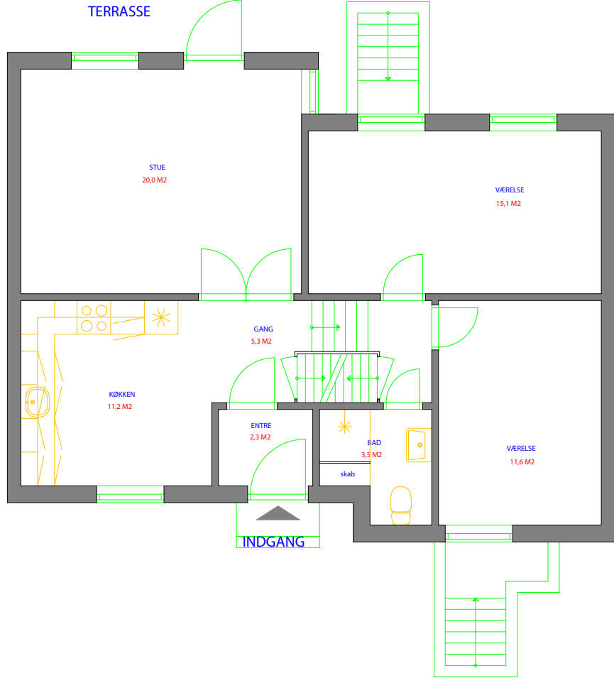
AFDELING 10 TYPE 32 3 RUMS 85 M2 STUEPLAN
